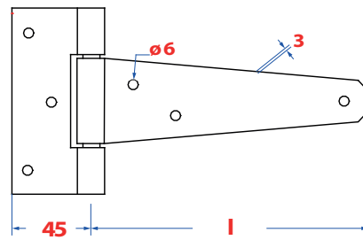
T-strap hinge
