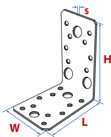
Square - Heavy type
