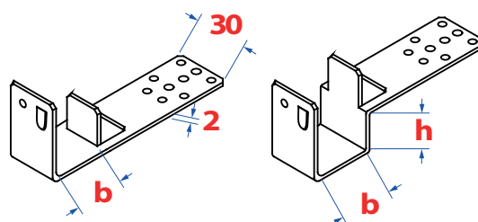
Rim shuttering anchor
