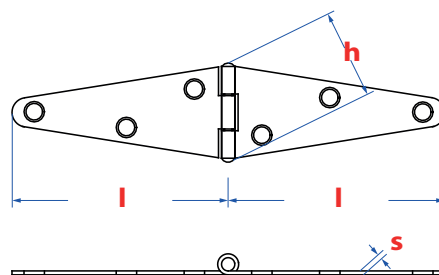
Straight strap hinge - Light version
