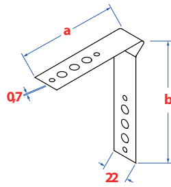
Spring anchor Federanker
