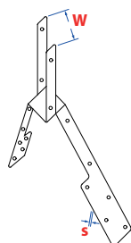
Ridge piece support
