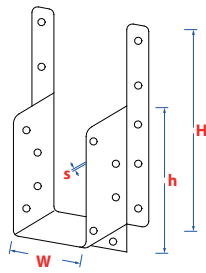
Joist hanger with strap
