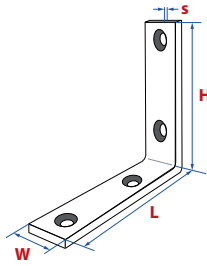
Narrow square
