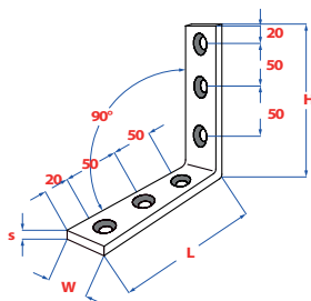
Cornice bracket - 90°
