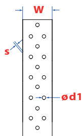
Straight assembly belt - 50 m
