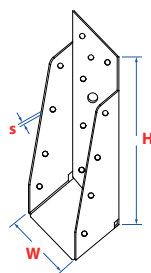
Beamsupport without lip
