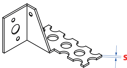
Frame anchor - l + r
